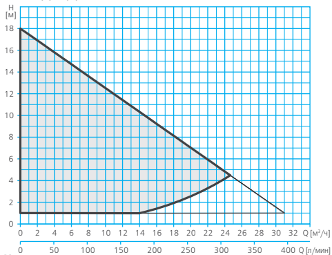
RV1(2)-F (X) 40-180
