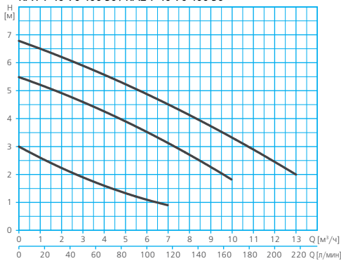
RA1-F 40-70 400 50 / RA2-F 40-70 400 50
