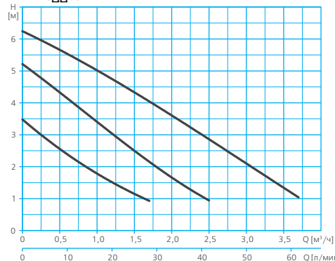
RA1-S...60
