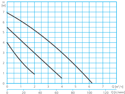
RA2-S 32-70-180 230 50
