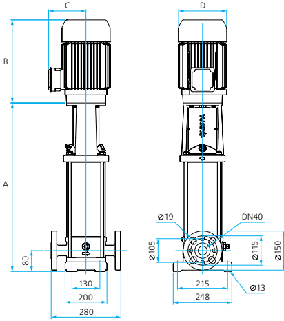
MULTI VX10
