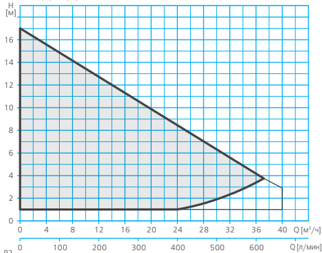
RV1(2)-F (X) 50-180
