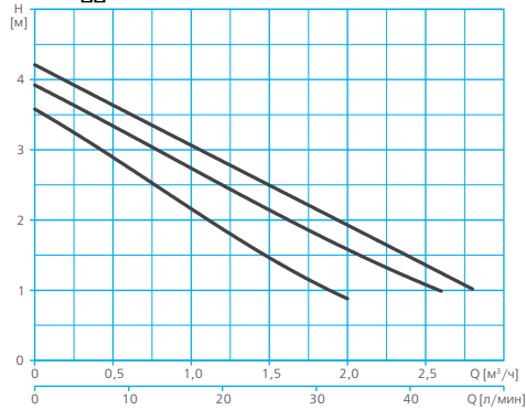
RA1-S...40
