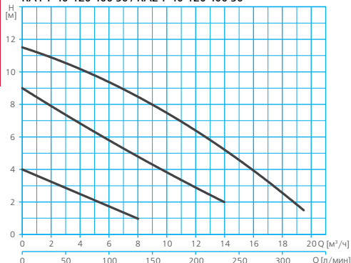
RA1-F 40-120 400 50 / RA2-F 40-120 400 50
