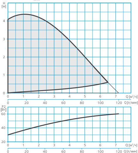
RE2-S(F) (X) _-40
