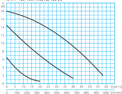
RA1-F 100-190-PN6(10) 400 50
