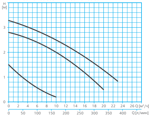
RA1-F 50-40 400 50 / RA2-F 50-40 400 50
